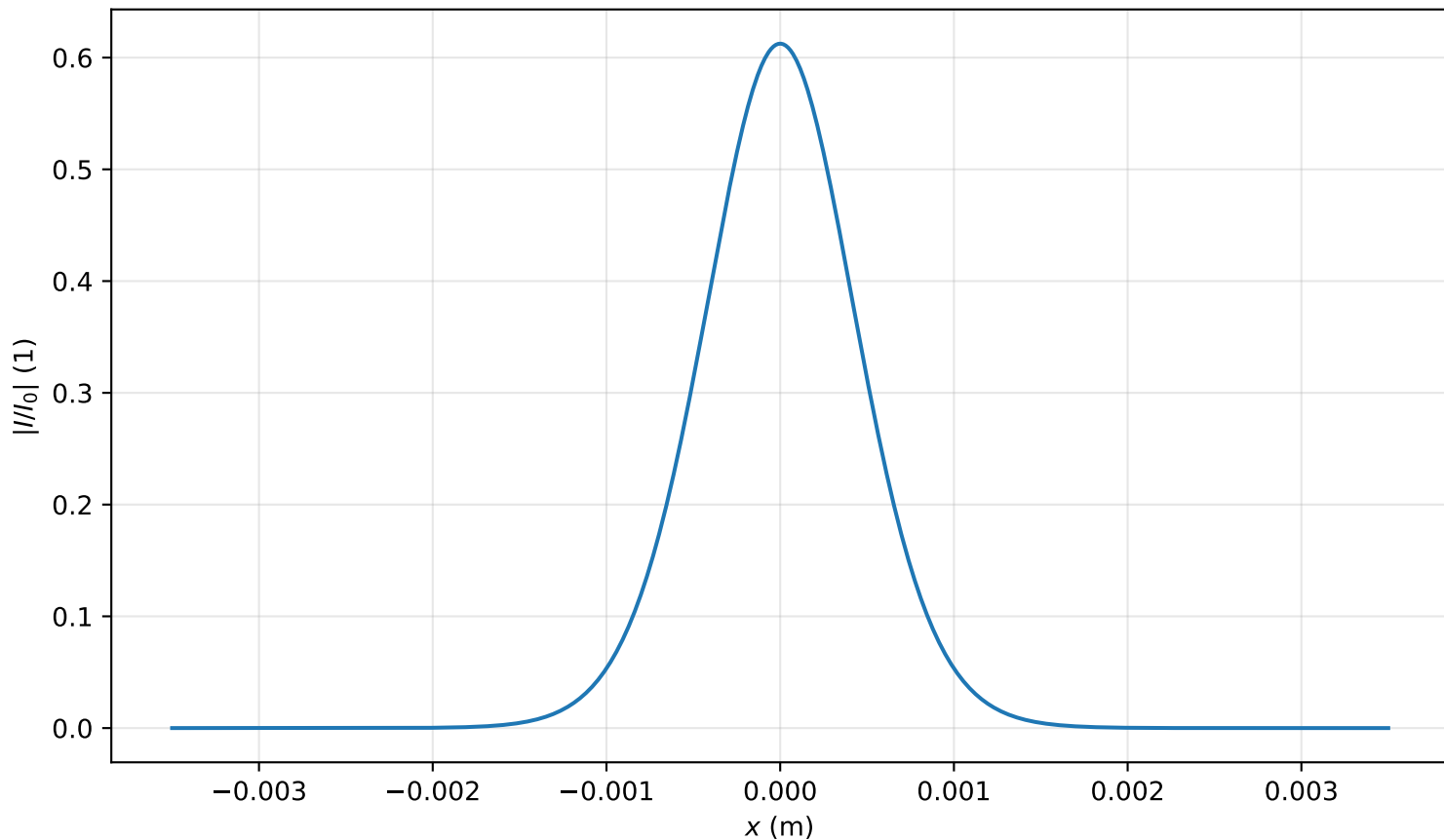
Intensity profile I(x, y = 0, z = 2.149m)/I_0 , P_{in}=0.3P_{cr} , artificial time
